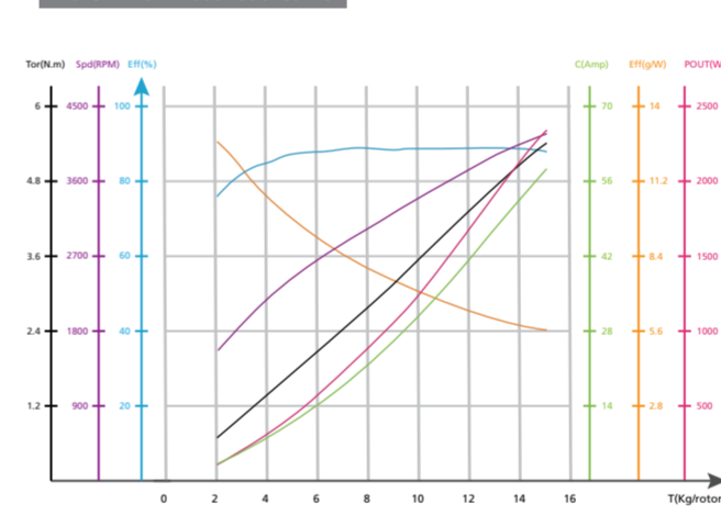
X8-G2-12S Thrust Load Curve
