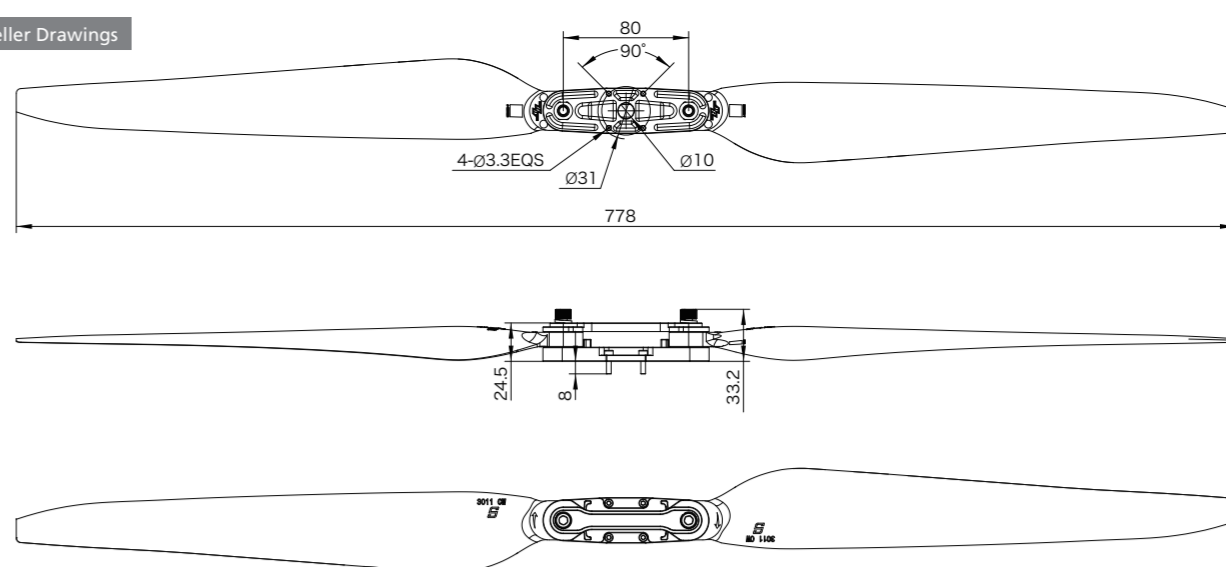
Propeller Drawings
