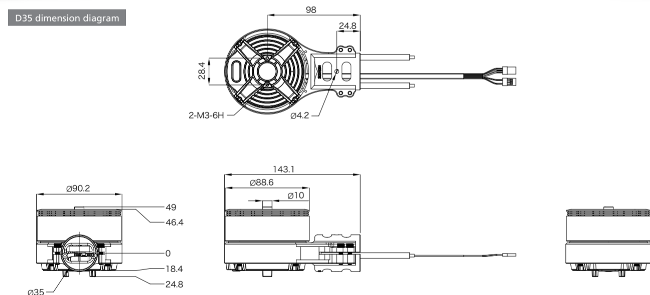
D35 dimension diagram
