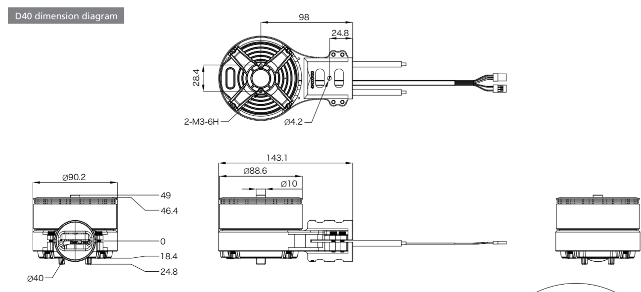
D40 dimension diagram
