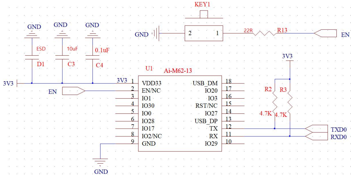
Figure 11 Application circuit diagram
