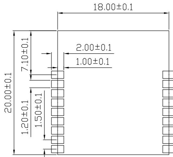
Figure 12 Recommend PCB footprint size
