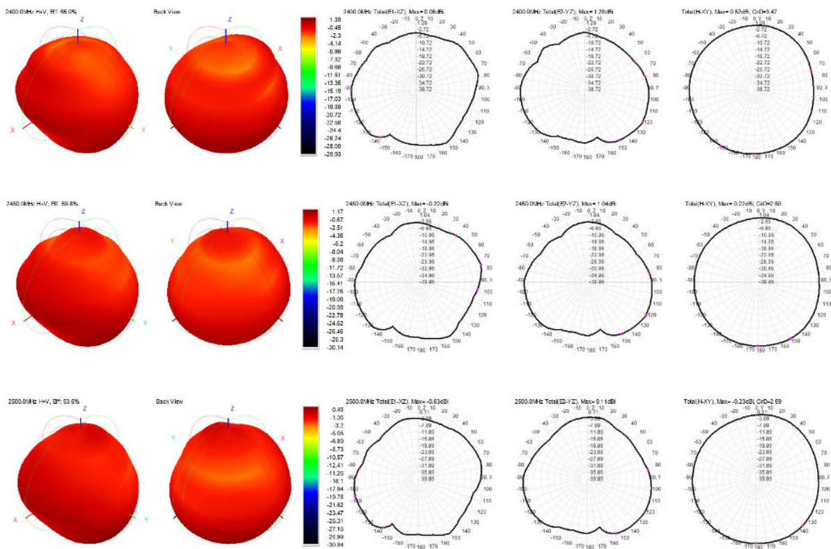
Figure 10 Antenna pattern
