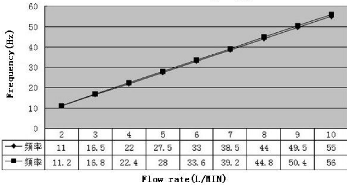
Flow rate vs. frequency plot
