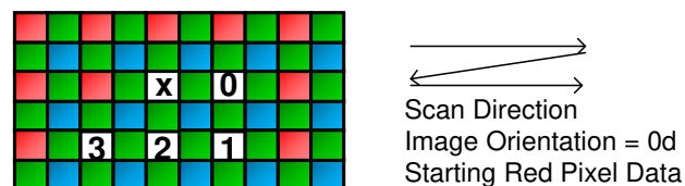
Fig. 36 Same Color Adjoining defect
