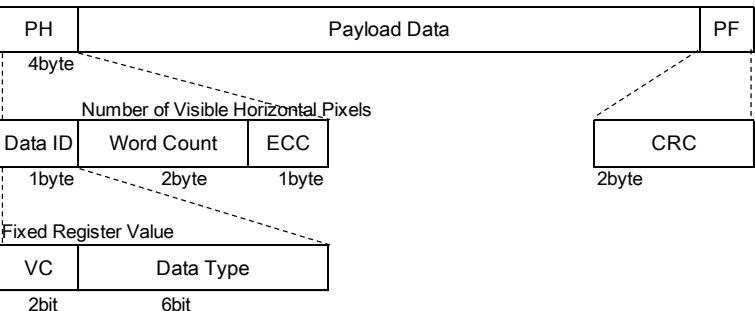
Fig. 23 Short Packet & Long Packet
