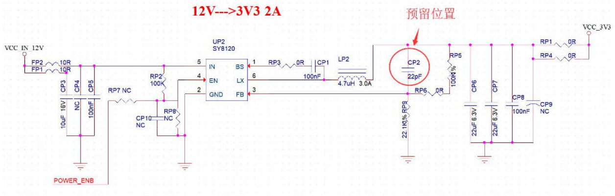
Figure 10 DC-DC Step-down circuit diagram
