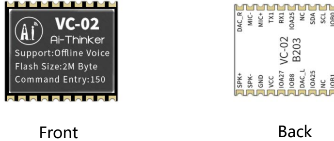
Figure 3 Module appearance diagram (For reference only)
