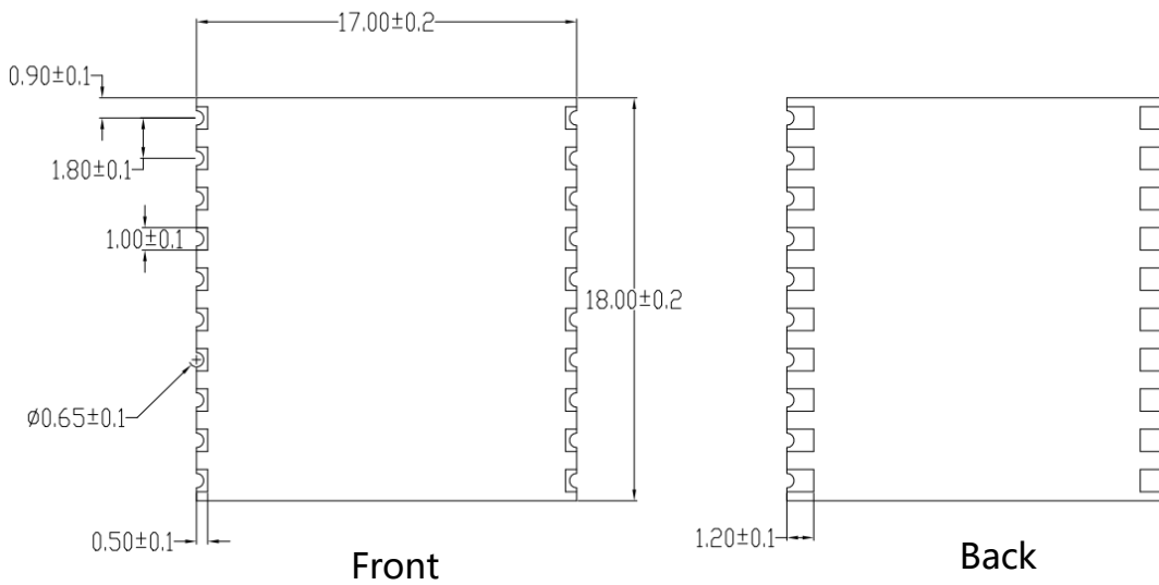
Figure 4 Module Size
